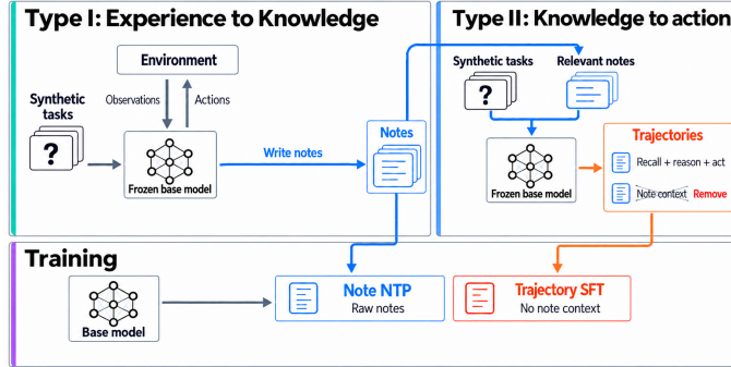
Figure 1: Overview of U-WIN. We generate two complementary types of synthetic data using a frozen base model in a new environment, without access to downstream test questions. Type I: Experience to Knowledge. The agent explores the environment on synthetic tasks and writes notes capturing what it learns. Type II: Knowledge to Action. We provide relevant notes in context and generate trajectories that interleave recalling this knowledge with reasoning and action. We then train on the note documents through next-token prediction and on the trajectories with the note context removed, after mixing with data of Type I.
