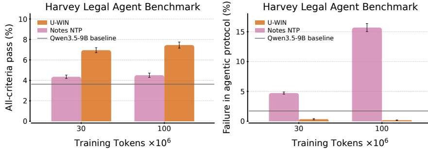
Figure 6: Type II data also preserves agentic behavior. Type I-only training (Notes NTP) vs. joint Type I+II training (U-WIN) on C&H at matched 30M and 100M token budgets. Left: joint training yields higher agentic task success. Right: protocol failures rise sharply with scale under Type I-only training but stay near the base model with joint training. Gray line: Qwen3.5-9B base model.
