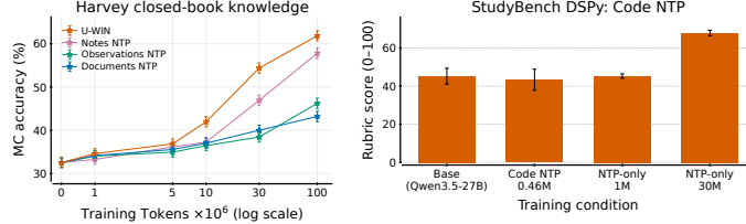
Figure 4: Left. Closed-book C&H knowledge accuracy as training data scales for U-WIN training, Type I notes, sampled environment documents, and interaction observations, all matched by token budget. Right. StudyBench agentic evaluation score vs training condition.
